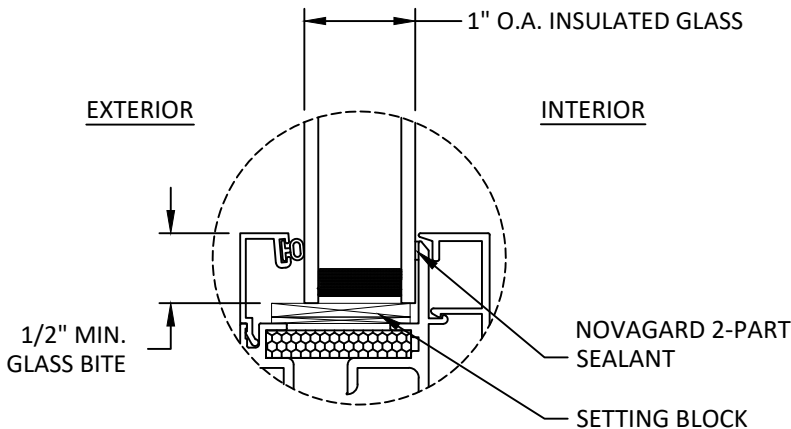
GLAZING DETAIL
