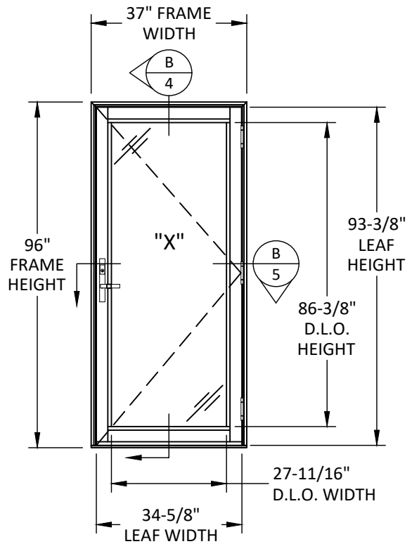
ELEVATION SINGLE OUTSWING
