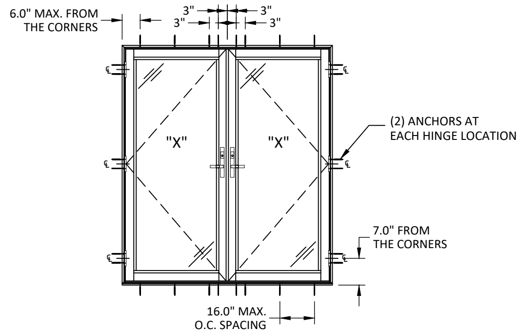
ANCHOR LAYOUT DOUBLE OUTSWING
