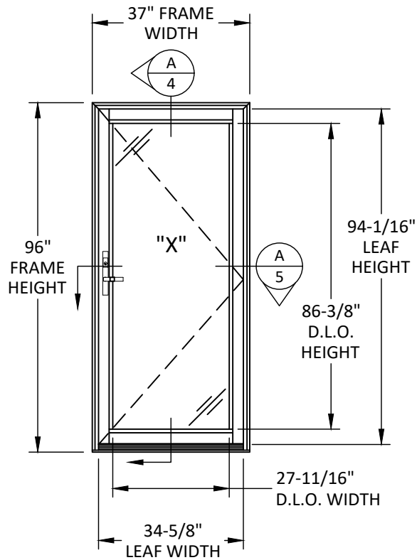
ELEVATION SINGLE INSWING
