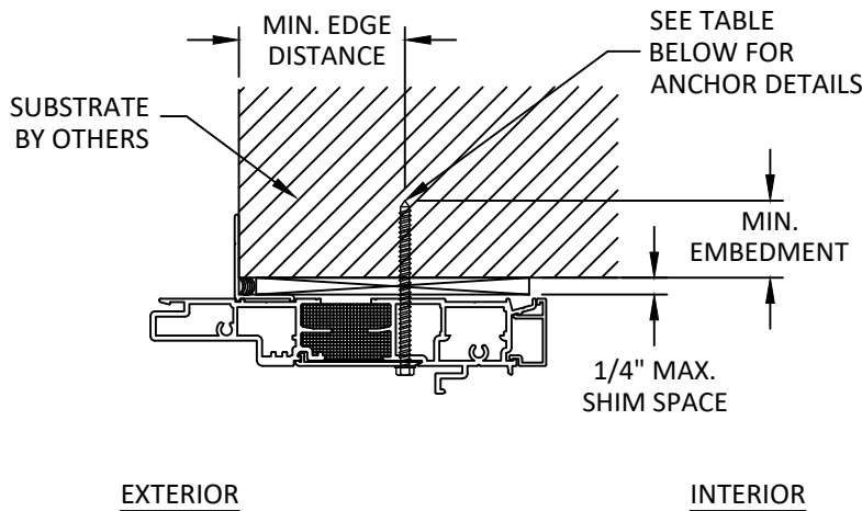
A 8 ANCHOR DETAIL OUTSWING HEAD NOTE: JAMB SIMILAR
