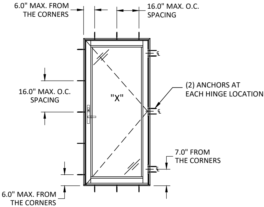
ANCHOR LAYOUT SINGLE OUTSWING
