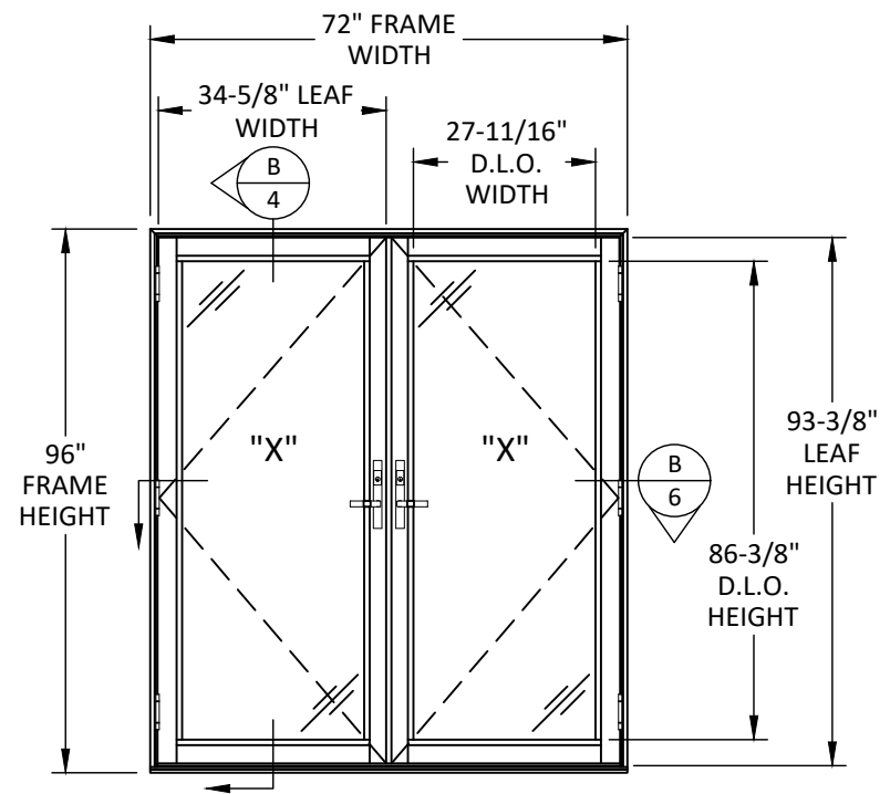
ELEVATION DOUBLE INSWING
