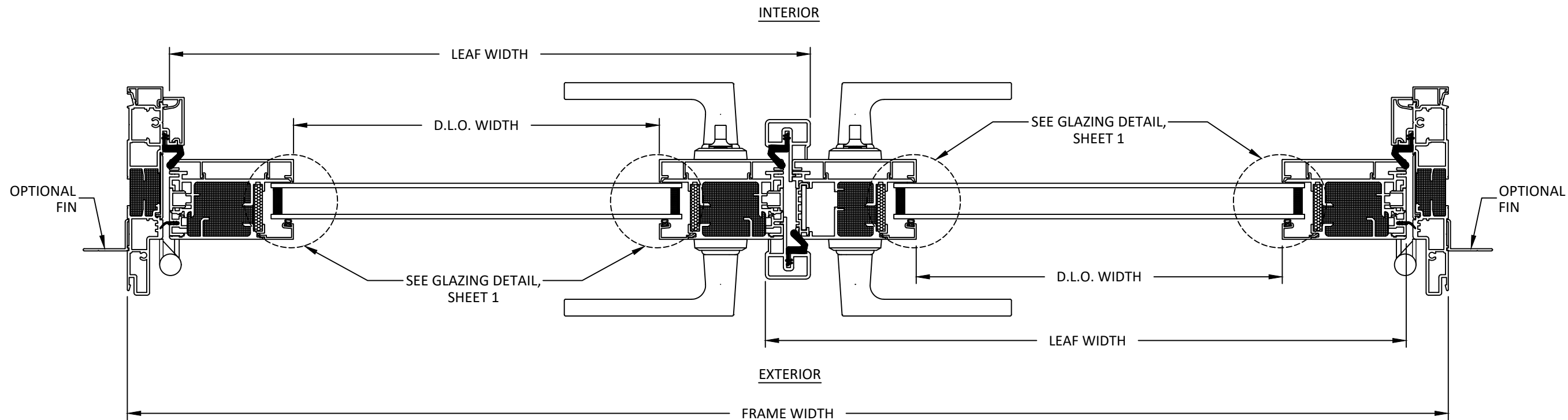
B 6 HORIZONTAL SECTION DOUBLE OUTSWING
