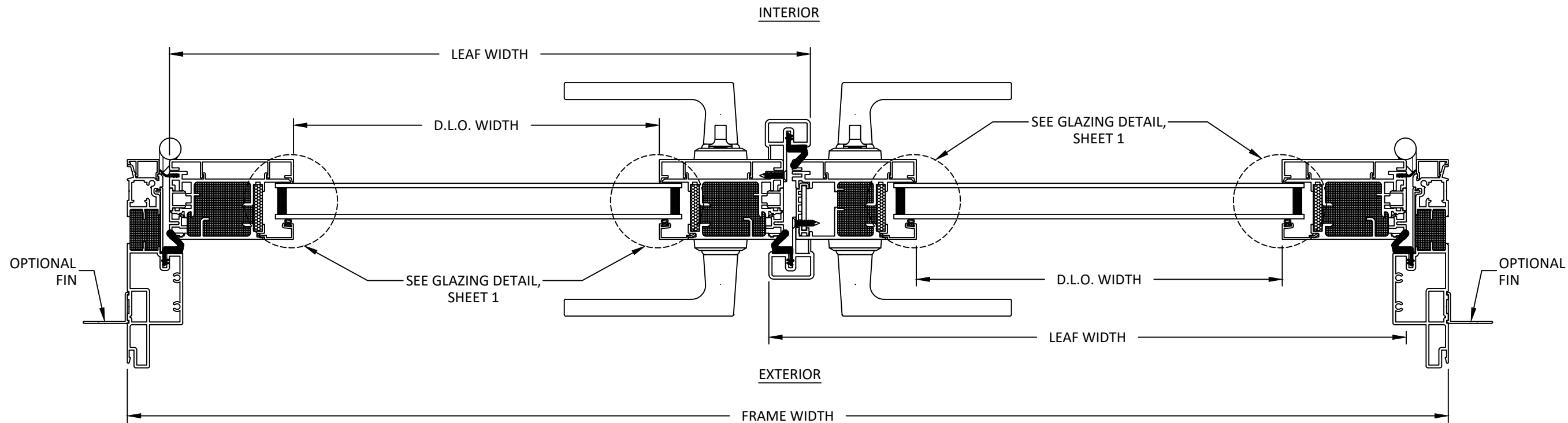
A 6 HORIZONTAL SECTION DOUBLE INSWING
