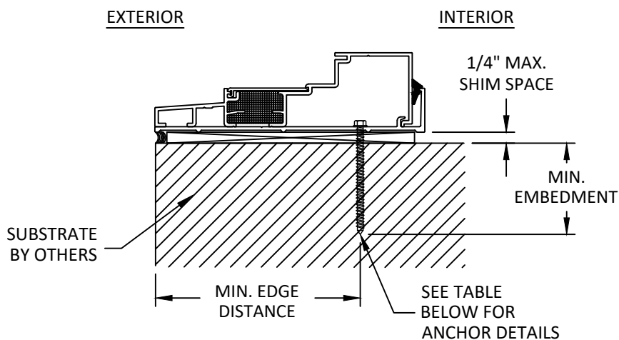
B 8 ANCHOR DETAIL OUTSWING SILL
