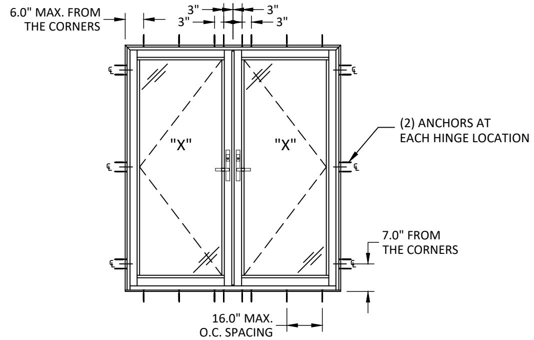
ANCHOR LAYOUT DOUBLE INSWING
